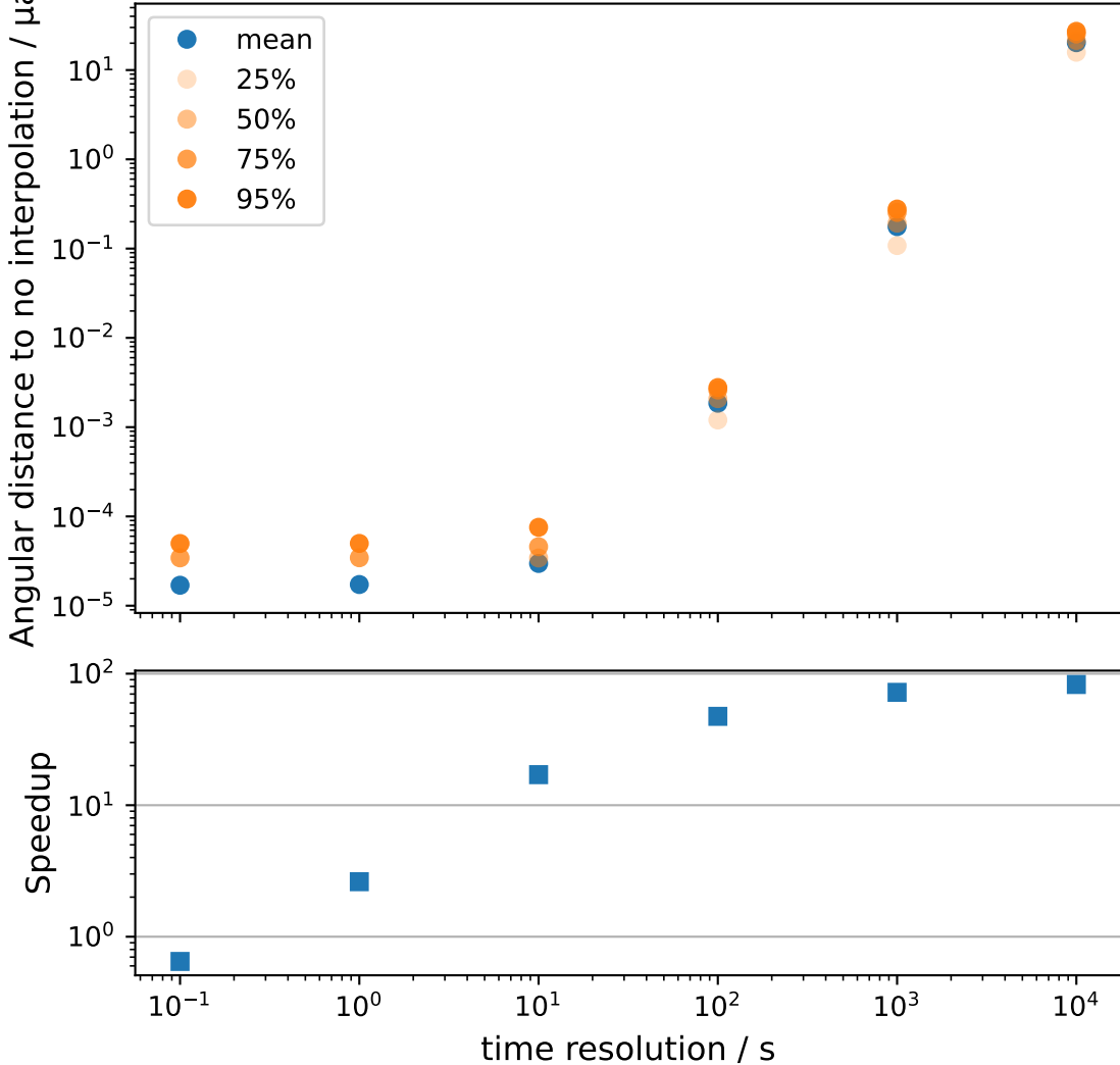
Transformation of SkyCoord with 10,000 obstimes over 1.0 h
