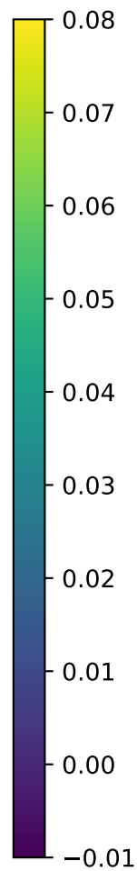
Gaussian2DKernel
