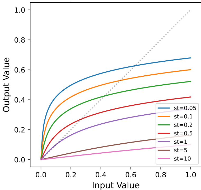
LuptonAsinhStretch, Q=10
